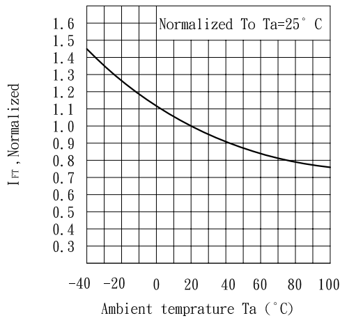
Fig. 9 Trigger Current vs. Ambient Temperature
