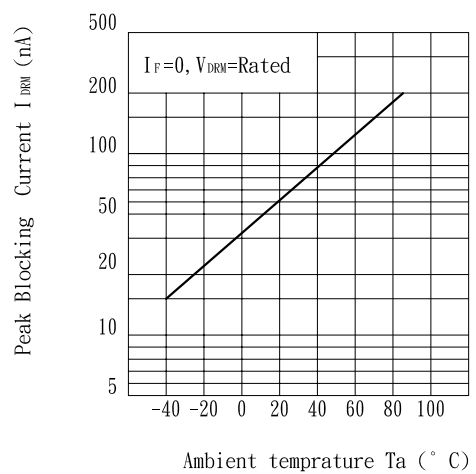
Fig. 8 Leakage with LED off vs. Ambient Temperature
