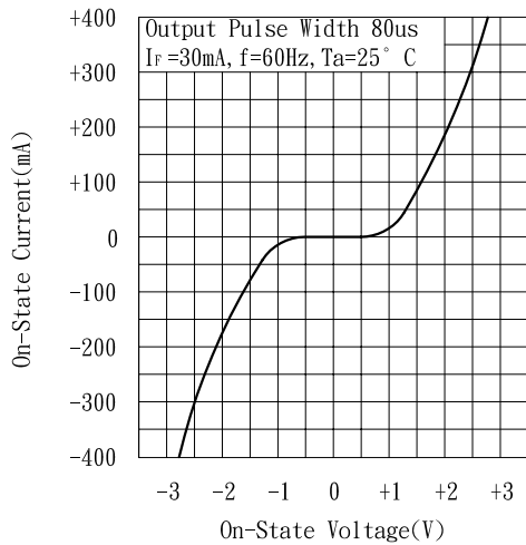
Fig. 7 On-State Characteristics
